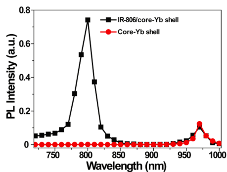
Figure 3. Excitation spectrum of \beta\text{-NaYF}_4\text{:}20\%\text{Yb}^{3+} , 2%Er 3+ @ \beta\text{-NaYF}_4\text{:}10\%\text{Yb}^{3+} (core/ \text{Yb}^{3+} active shell) nanoparticle with (black squares) and without (red circles) IR-806 dye sensitization.
