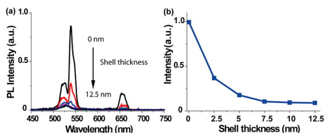
Figure 1. (a) Emission spectra of IR-806-dye-sensitized UCNPs exhibiting various \beta\text{-NaYF}_4 shell thickness (i.e., 0, 2.5, 5, 7.5, 10, and 12.5 nm, respectively) upon 800 nm CW laser excitation. (b) The integrated emission peak area (from 500 to 700 nm) of those dye-sensitized UCNPs decreases as the shell thickness increases. Note: In order to guide the eye, the data points are connected by lines.
