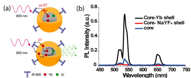
Figure 2. (a) Schematic showing the proposed energy transfer mechanism for core/shell UCNPs without (top) and with (bottom) \text{Yb}^{3+} doping. (b) Emission spectra of IR-806-sensitized core only ( \beta\text{-NaYF}_4\text{:}20\%\text{Yb}^{3+} , 2%Er 3+ ), core/ \text{NaYF}_4 shell ( \beta\text{-NaYF}_4\text{:}20\%\text{Yb}^{3+} , 2%Er 3+ @ \beta\text{-NaYF}_4 ), core/ \text{Yb}^{3+} shell ( \beta\text{-NaYF}_4\text{:}20\%\text{Yb}^{3+} , 2%Er 3+ @ \beta\text{-NaYF}_4\text{:}10\%\text{Yb}^{3+} ). Note: The shell exhibited a controlled thickness of \sim 7.5\text{ nm} for core/ \text{NaYF}_4 shell and core/ \text{Yb}^{3+} shell UCNPs. The measurements were performed under 800 nm continuous wave laser excitation ( 2\text{ W/cm}^2 ), with a UCNP concentration of 0.1\ \mu\text{mol/L} (ET: energy transfer).
